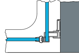
Detail A – pôdorys
