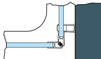
Detail A - pôdorys
